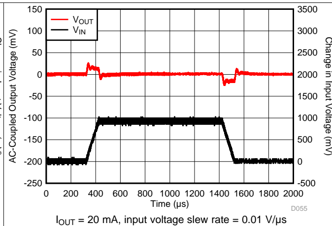
Figure 20. V_{IN} Transient
