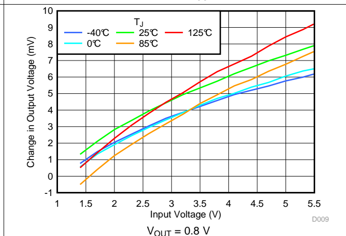
Figure 24. Line Regulation V_{IN} and Temperature
