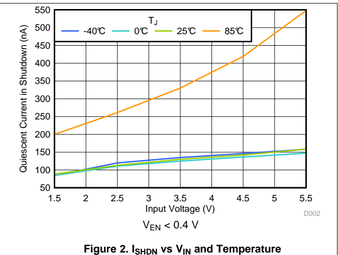
Figure 2. I_{SHDN} vs V_{IN} and Temperature
