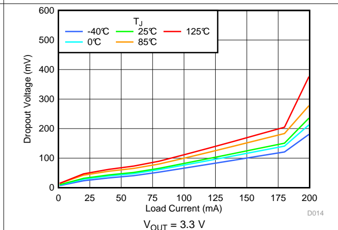
Figure 22. Dropout vs I_{OUT} and Temperature
