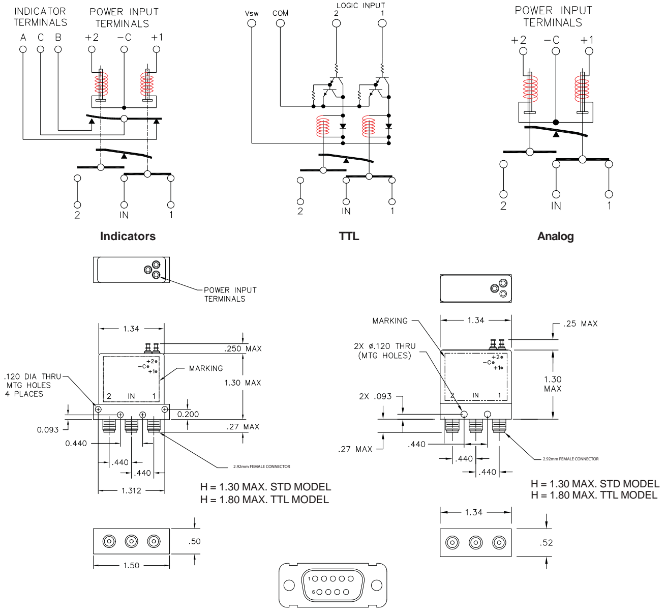
“-S OPTION” 9-PIN D-SUB CONNECTOR (EXAMPLE: CCR-33K60-S)
