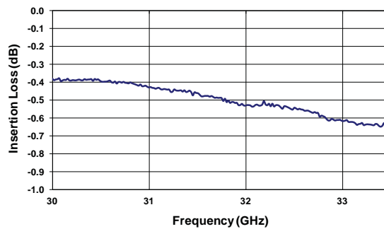
Insertion Loss (30-33.5 GHz)
