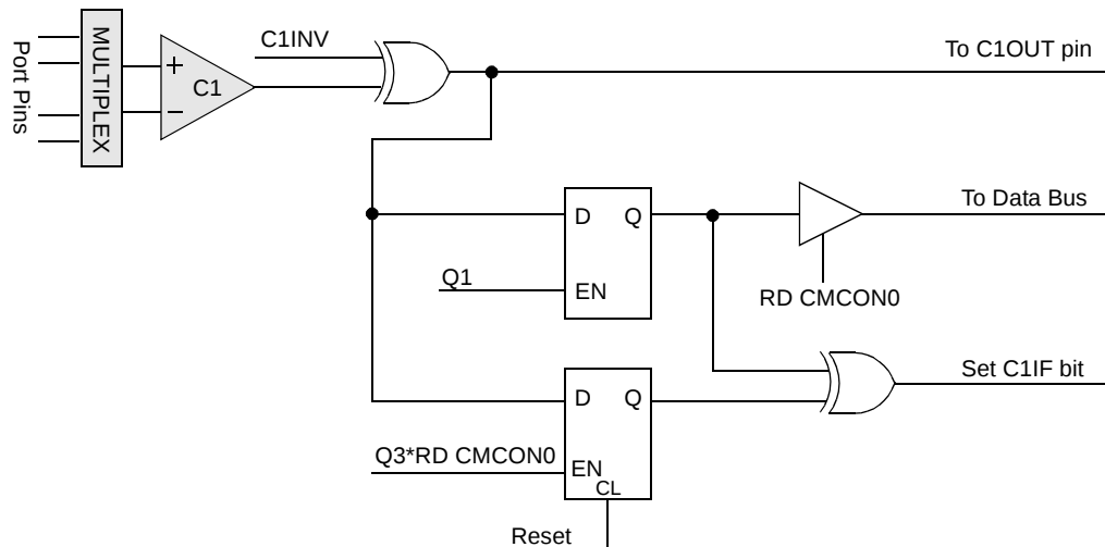
FIGURE 7-2: COMPARATOR C1 OUTPUT BLOCK DIAGRAM
