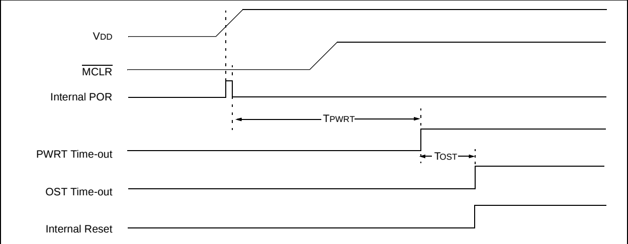
FIGURE 11-5: TIME-OUT SEQUENCE ON POWER-UP (DELAYED \overline{\text{MCLR}} )
