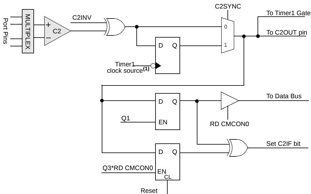
FIGURE 7-3: COMPARATOR C2 OUTPUT BLOCK DIAGRAM
