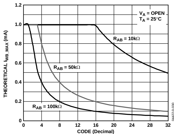
Figure 29. Maximum I_{WB} vs. Code
