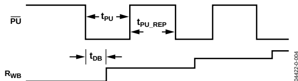
Figure 2. Increment R_{WB} in Discrete Steps
