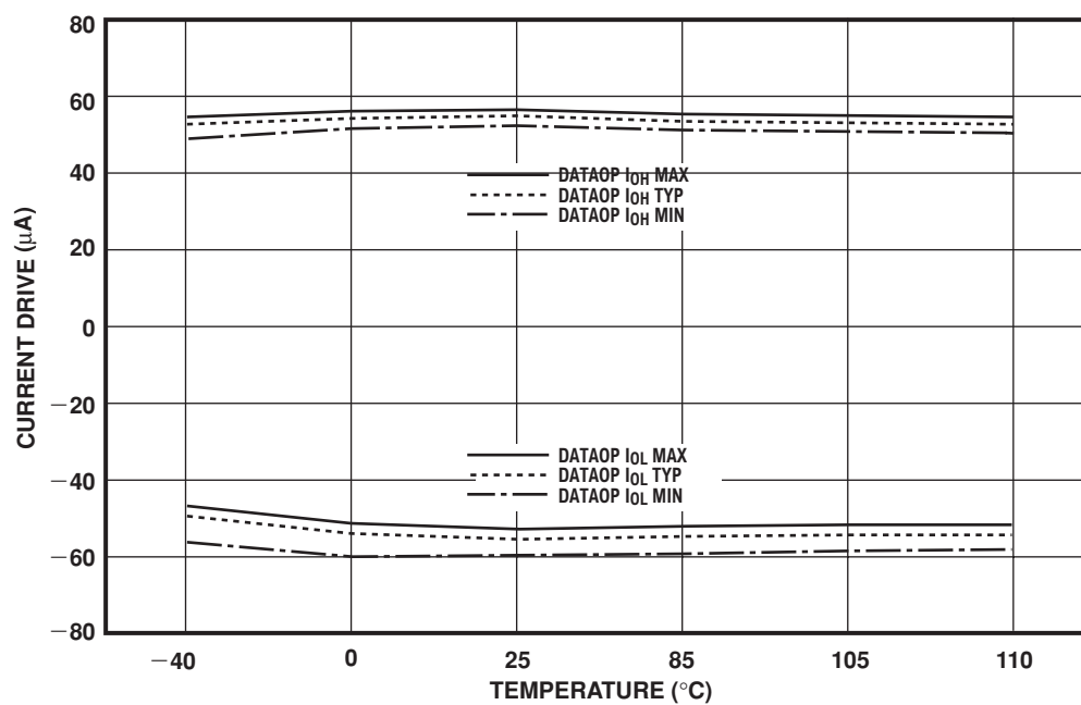
Figure 21 DATAOP I/O current drive at \pm 20\mu\text{A} (see Baseband, page 13)
