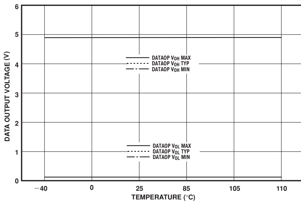
Figure 20 DATAOP I/O voltage drive at \pm 20\mu\text{A} ( V_{OH}/V_{OL} , AC Electrical Characteristics (1), page 7)
