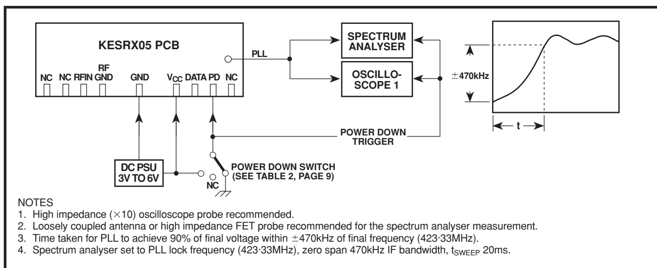
Figure 7 Characterising the PLL acquisition time from power-up
