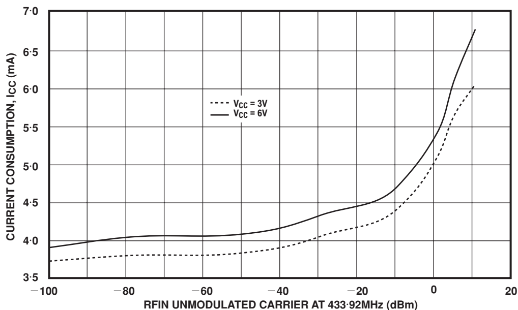
Figure 16 Receiver current consumption v. received signal strength RFIN (see RF Down-converter, page 9)
