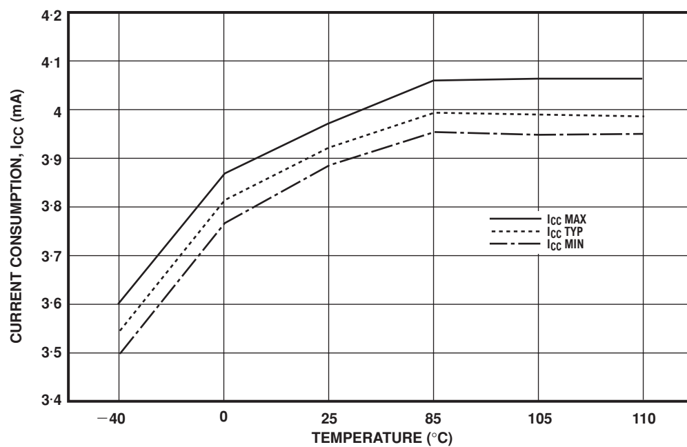
Figure 24 Receiver current consumption in PD2 mode, DC Electrical Characteristics, page 7
