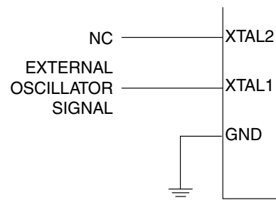
Figure 25. External Clock Drive Configuration
