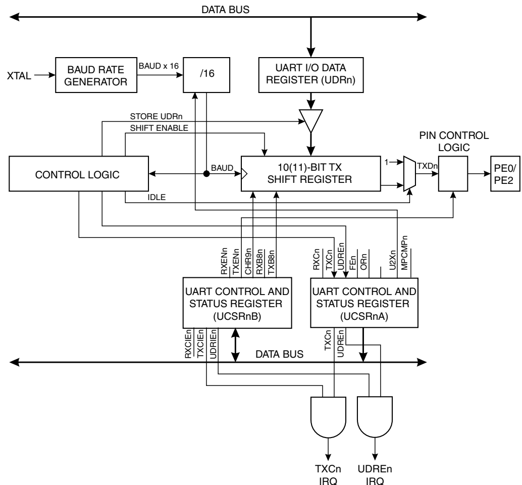
Figure 64. UART Transmitter (1)
