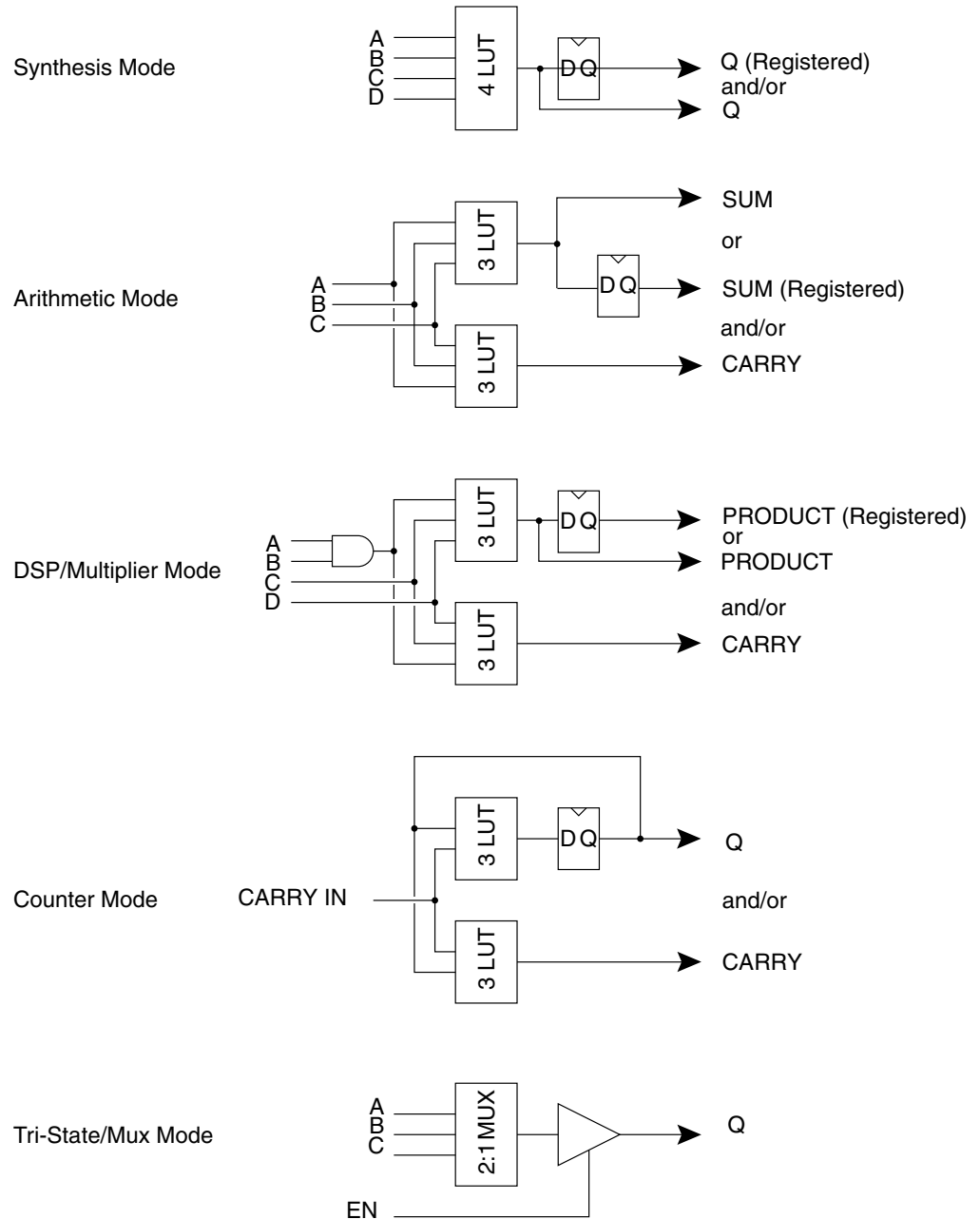
Figure 7. Some Single Cell Modes
