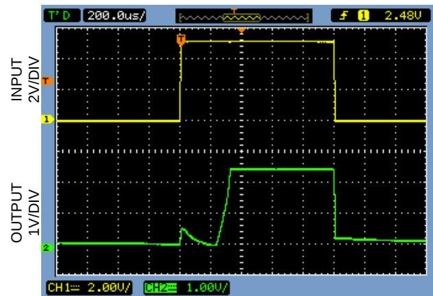
Power-On Transient Response
