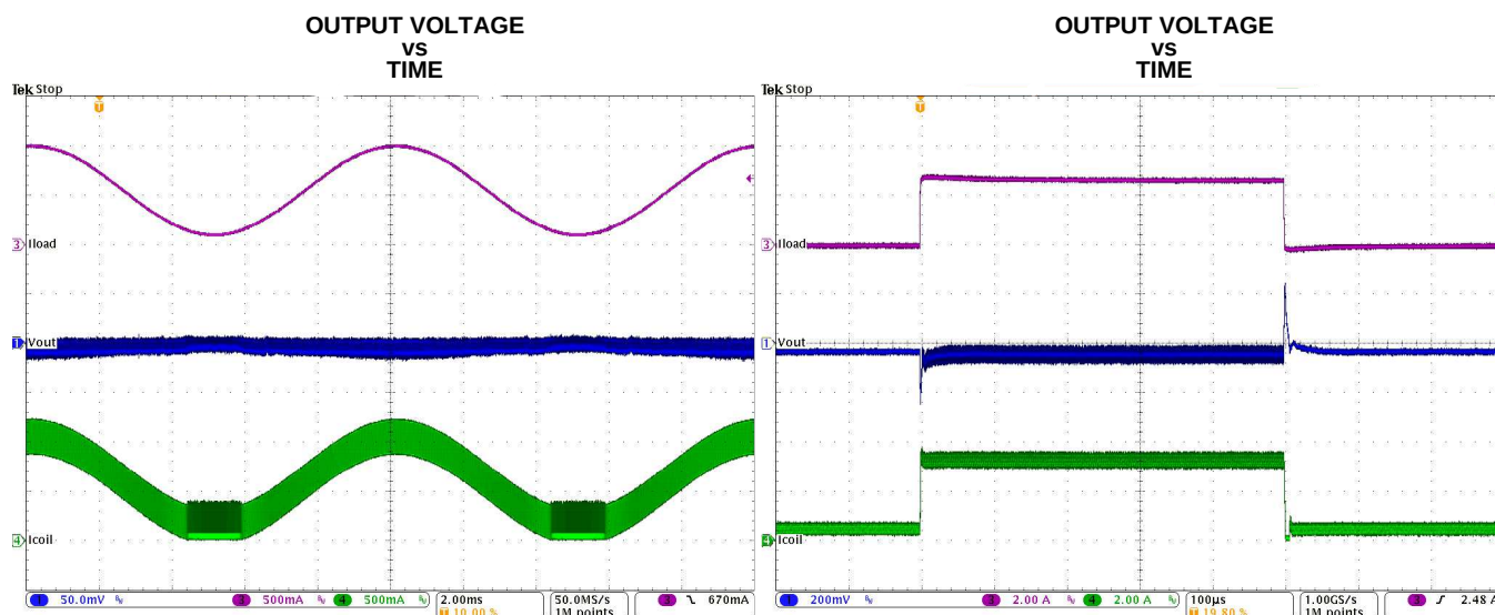
Figure 29. PWM-PSM-Transition ( V_{IN}=12V , V_{OUT}=3.3V with 50mV/div)
