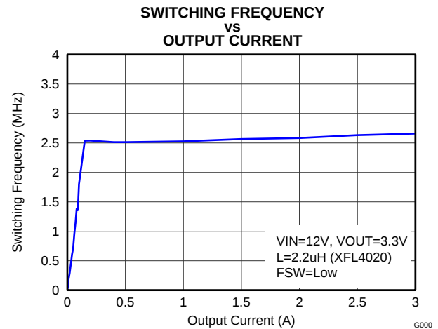
Figure 20. Switching Frequency
