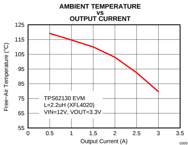
Figure 37. Maximum Ambient Temperature ( f_{SW}=2.5\text{MHz} )
