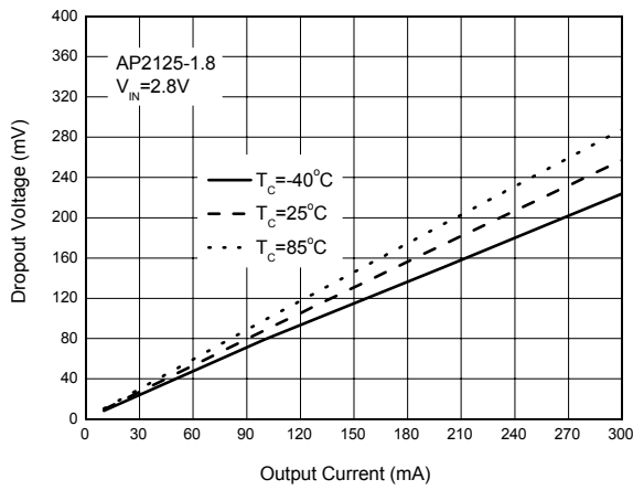
Figure 6. Dropout Voltage vs. Output Current
