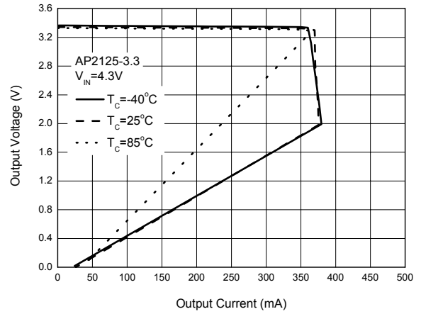
Figure 13. Current Limit
