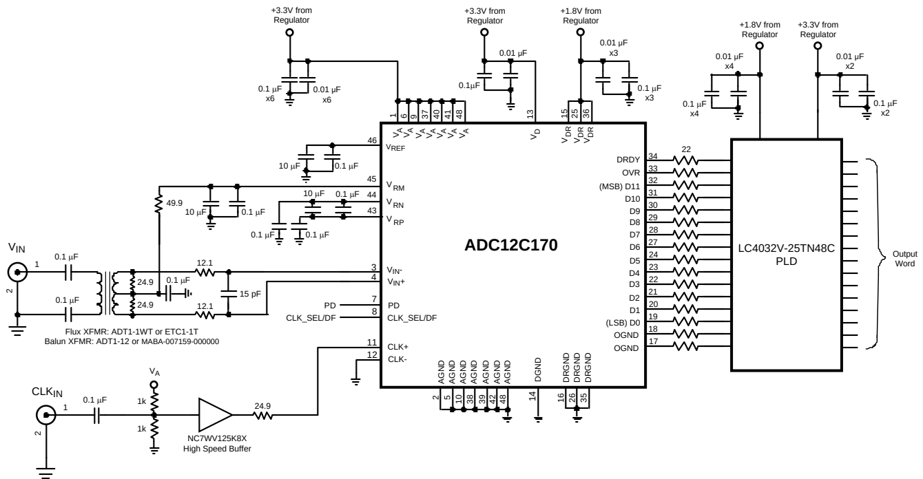
Figure 23. Application Circuit using Transformer Drive Circuit (If 14-bit compatibility is not required do not connect pins 17 and 18)
