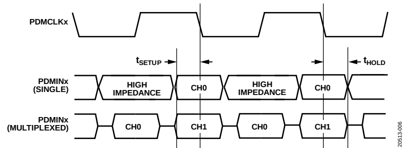
Figure 6. PDM Input Timing Diagram
