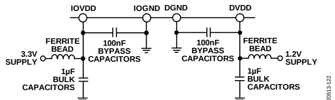
Figure 24. Ferrite Bead Power Supply Isolation Circuit
