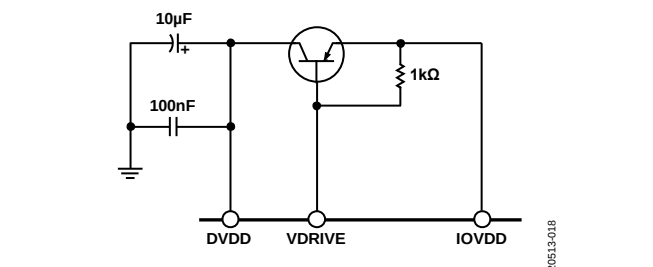
Figure 20. External Components Required for Voltage Regulator Circuit
