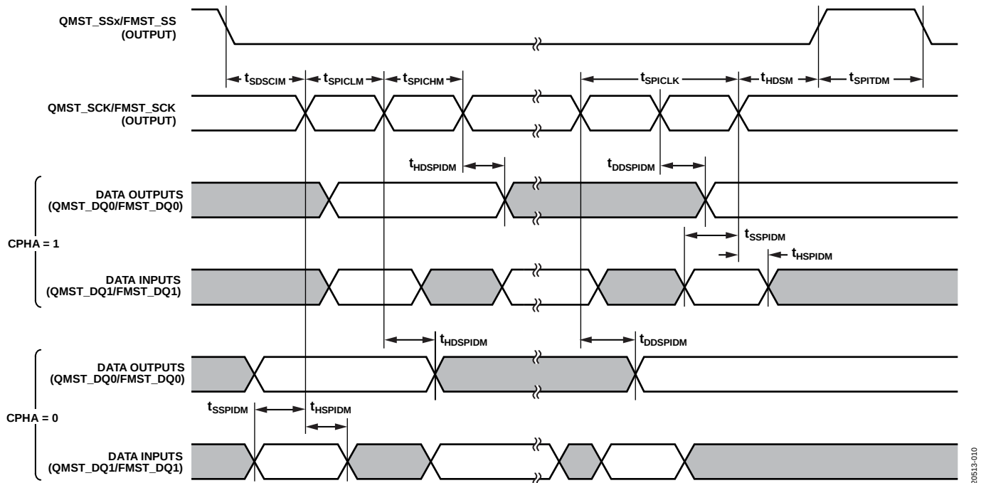
Figure 10. SPI Master Port Timing Specifications
