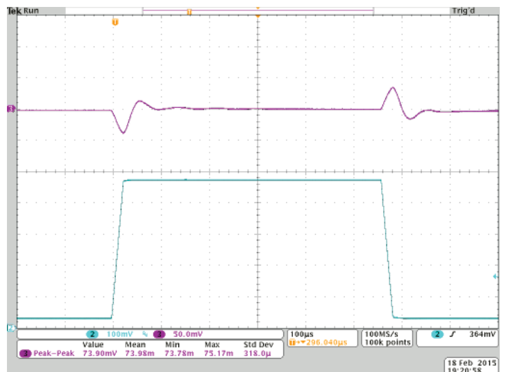
Transient Response
