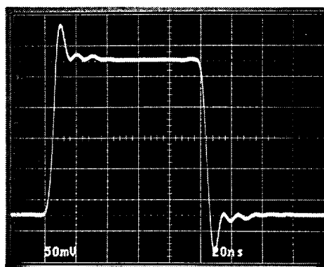
A_V = -1 , IN DEMO BOARD, C_L = 30\text{pF} WITH 10 \Omega ISOLATING RESISTOR
