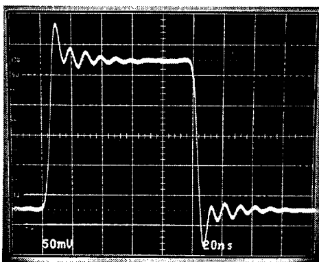
A_V = -1 , IN DEMO BOARD, C_L = 30\text{pF}
