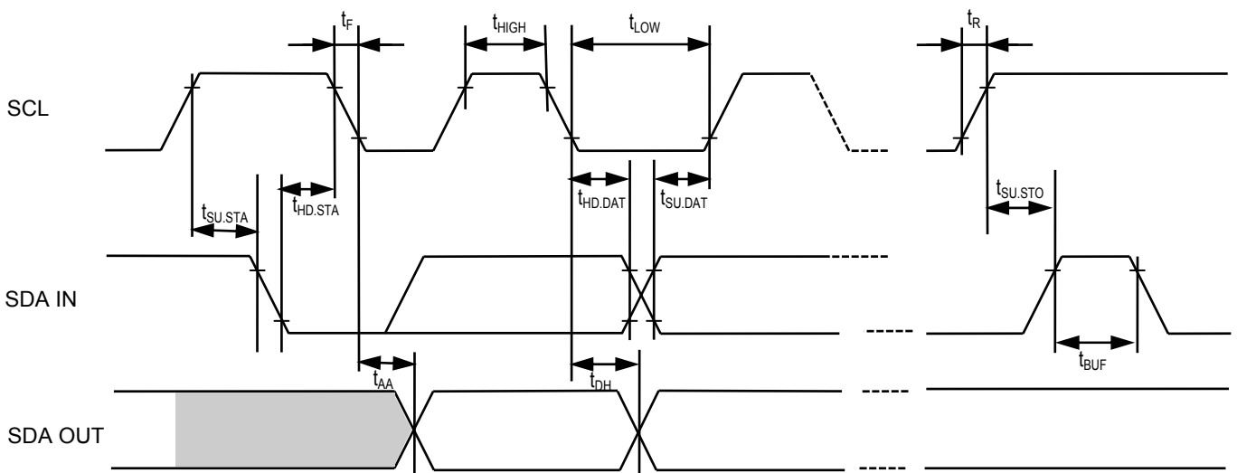
Figure 11 Bus Timing
