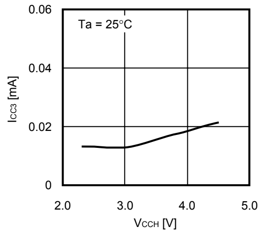
1. 12 Internal oscillator current consumption during operation I_{CC3} vs. Power supply voltage V_{CCH}
