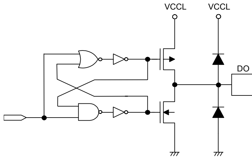
Figure 9 DO Pin
