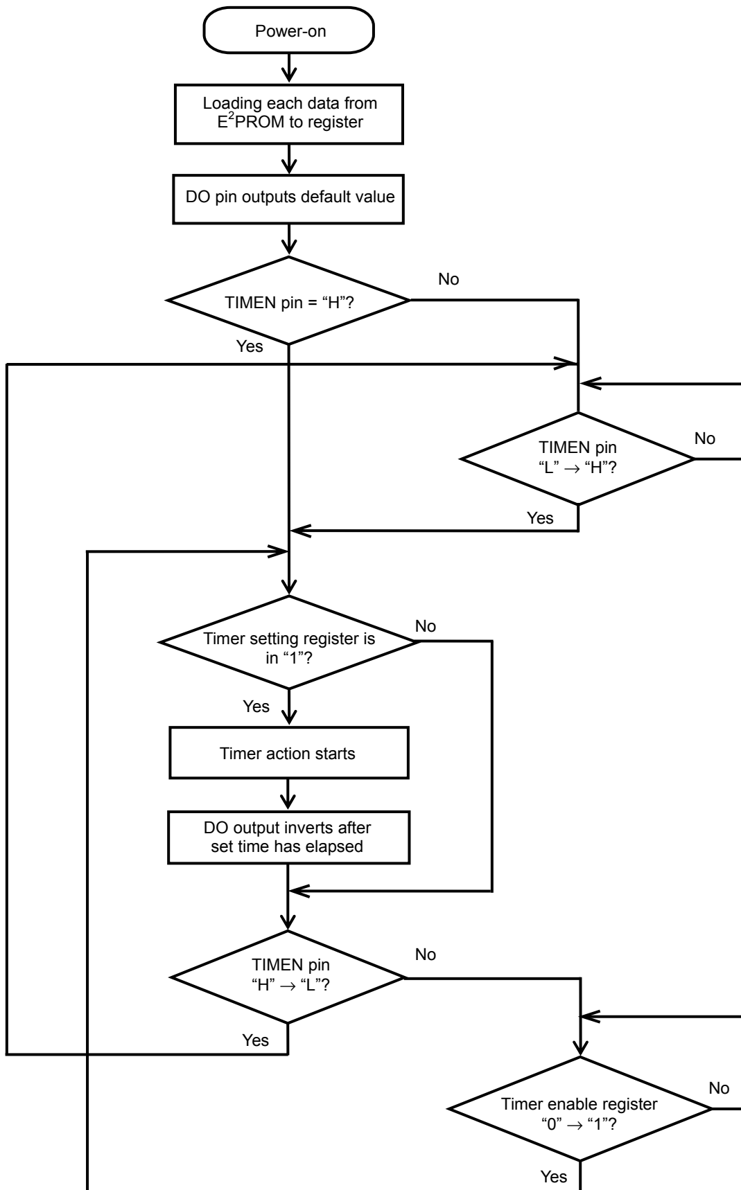
Figure 21 Flowchart of S-7760A's Action (When selecting "condition to start timer Option 1")
