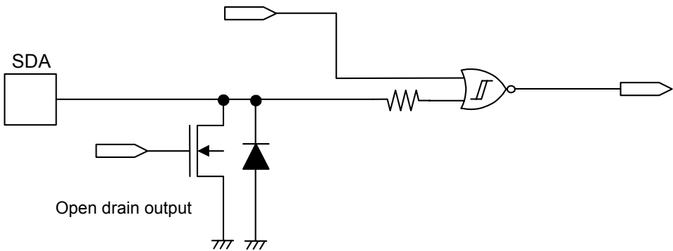
Figure 7 SDA Pin
