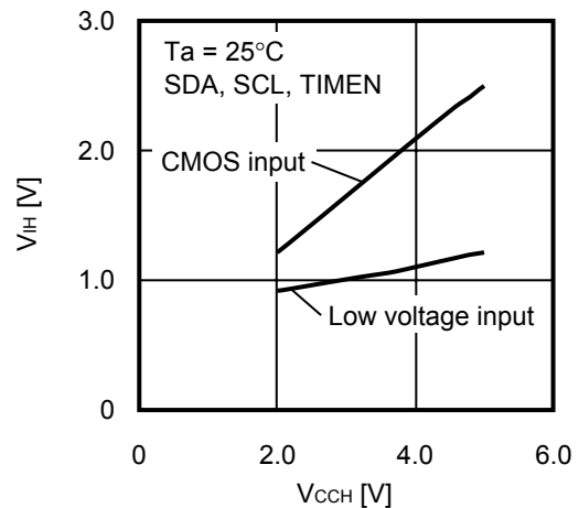
1. 30 High level input inversion voltage V_{IH} vs. Power supply voltage V_{CCH}
