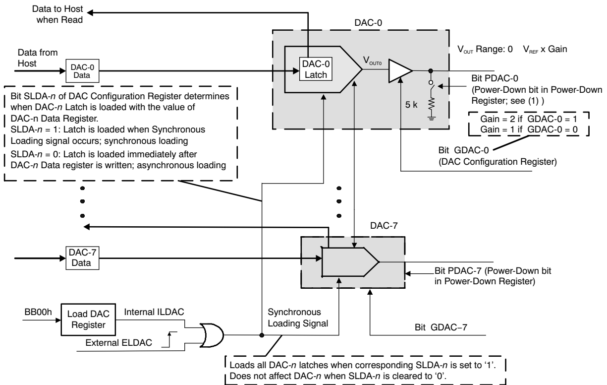
Figure 47. DAC Structure
