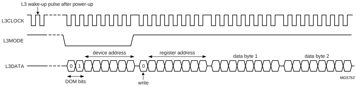
Fig.6 Data write mode (for L3-bus version 2).
