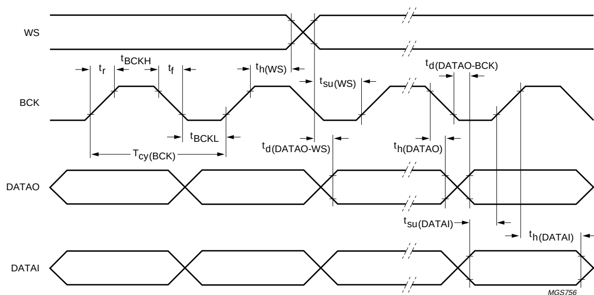
Fig.17 Serial interface input/output data timing.
