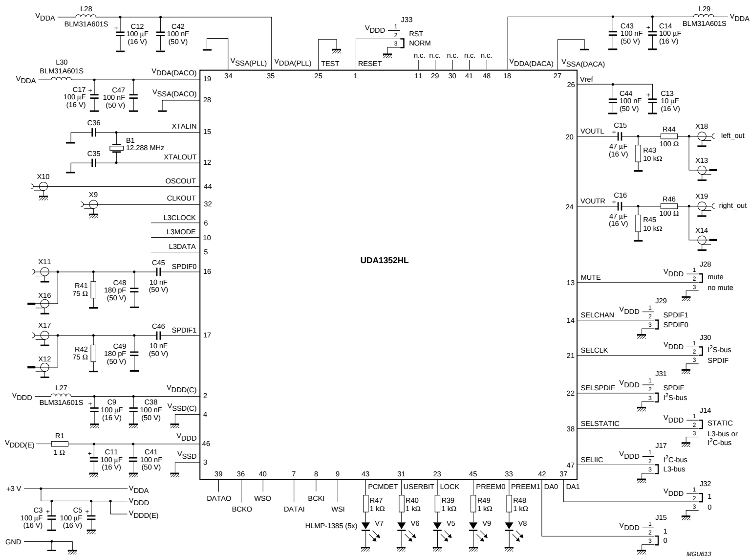
Fig.21 Application diagram.
