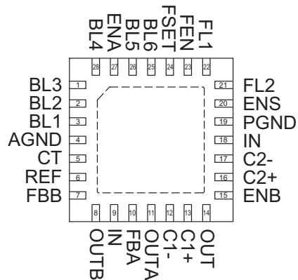
TQFN44-28 (Top View)
