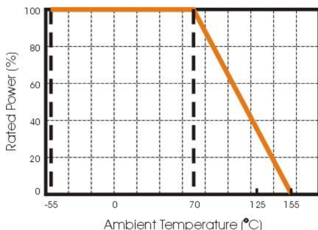
Fig 3 Maximum dissipation in percentage of rated power as a function of the ambient temperature
