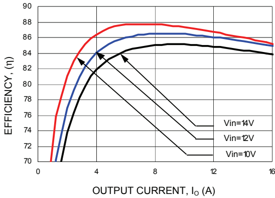
Figure 1. Converter Efficiency versus Output Current (V out = 1.2Vdc).
