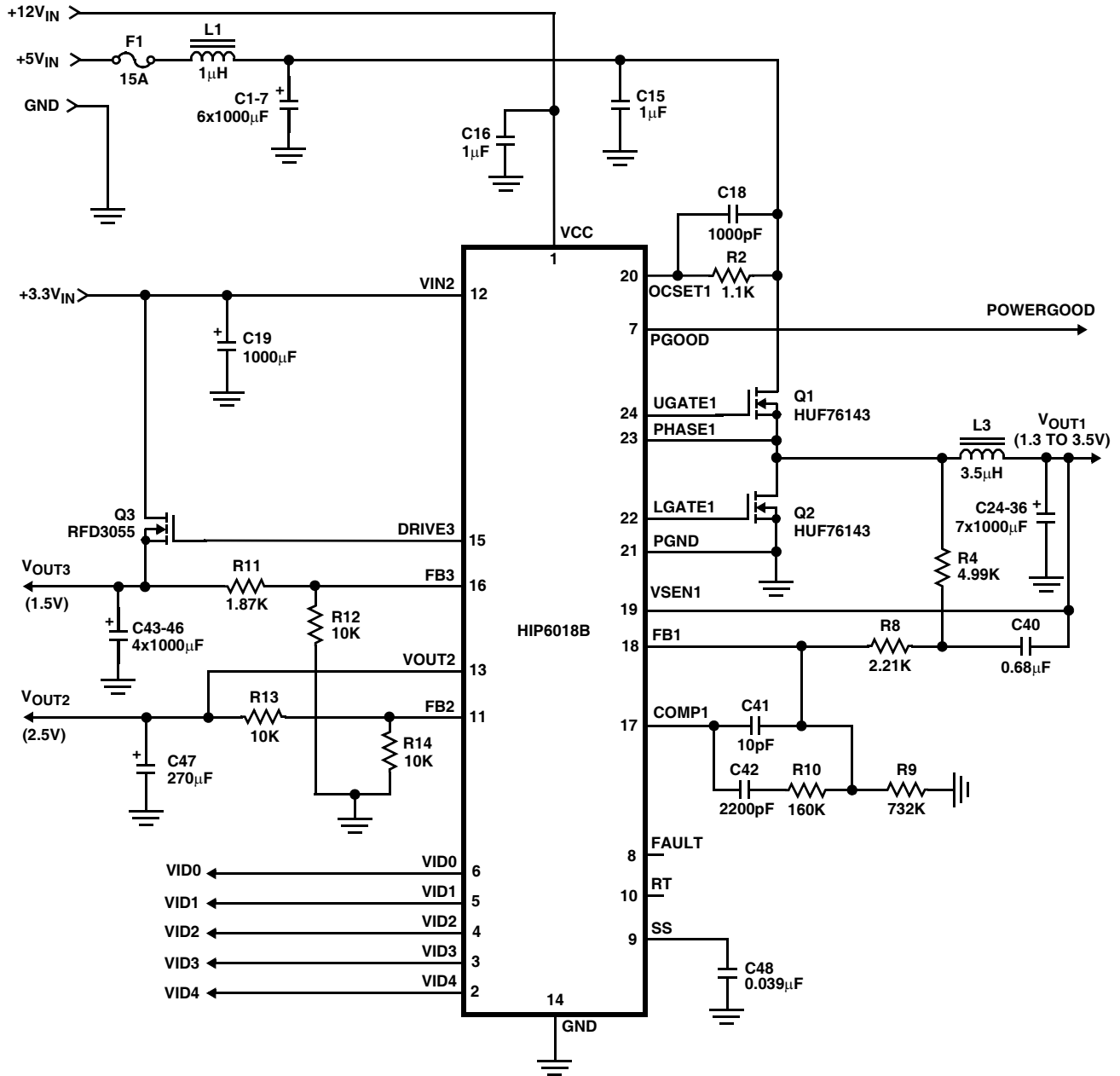
FIGURE 15. APPLICATION CIRCUIT
