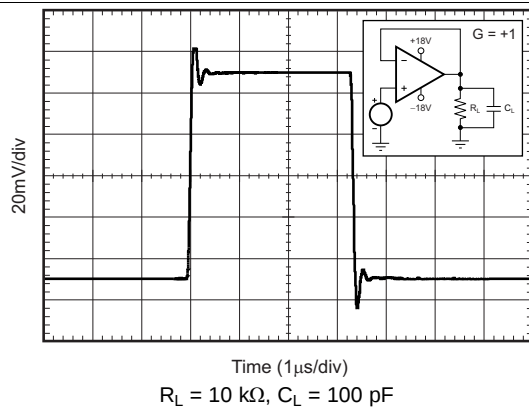
Figure 17. Small-Signal Step Response (100 mV)
