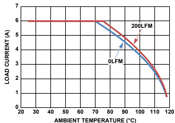
FIGURE 30. DERATING CURVES AT V_{IN} = 3.3V , V_{OUT} = 2.5V
