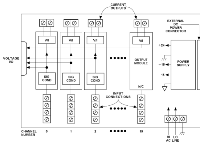
Figure 1 3B01 Functional Block Diagram
