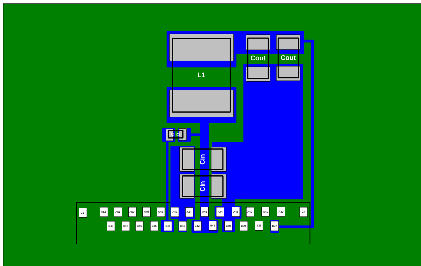
Figure 71. DCDC1 Layout Example
