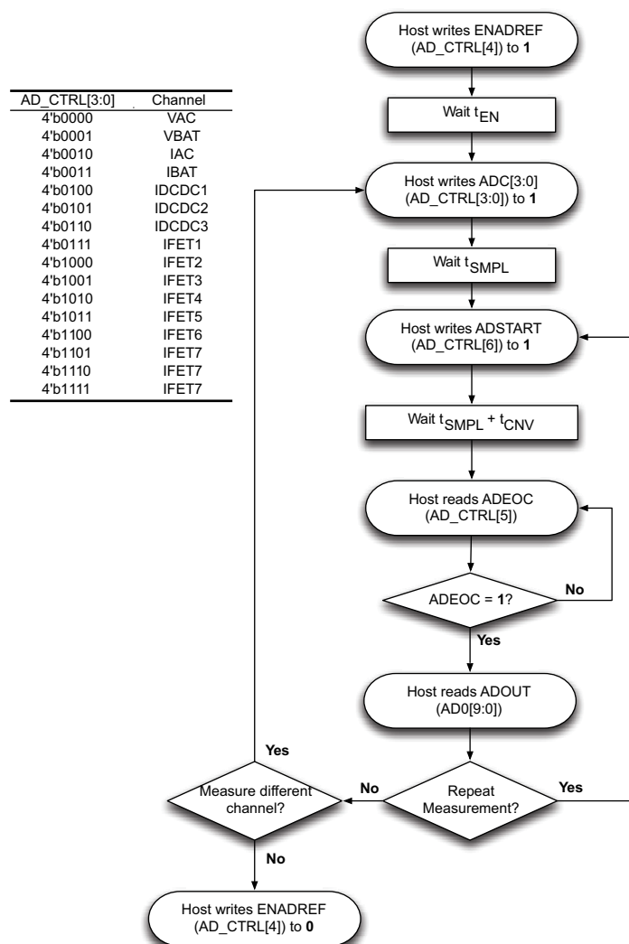
Figure 39. Analog-to-Digital Conversion
