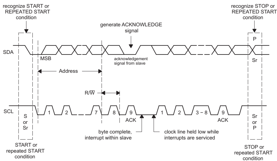
Figure 43. Bus Protocol
