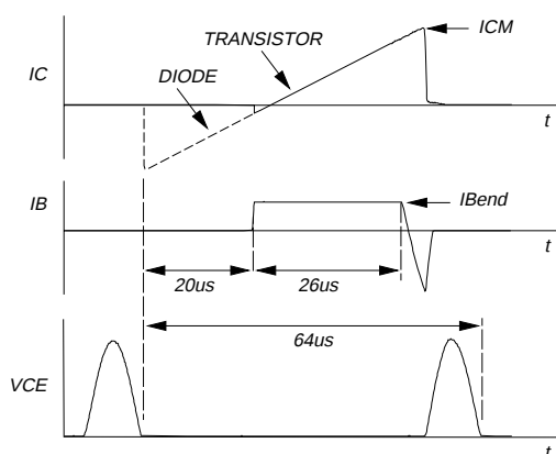
Fig.3. Switching times waveforms (16 kHz).
