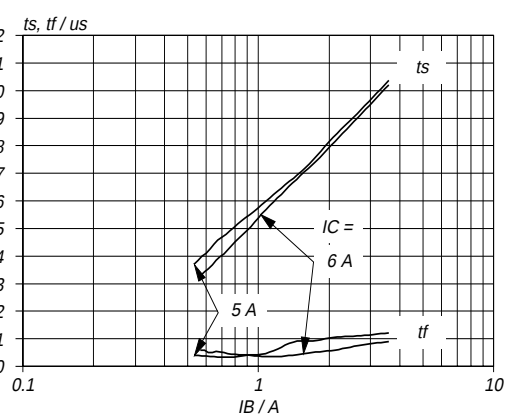
Fig.13. Typical collector storage and fall time. t_s = f(I_B) ; t_f = f(I_B) ; parameter I_C ; T_j = 85^\circ\text{C} ; f = 16\text{ kHz}
