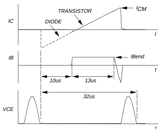
Fig.4. Switching times waveforms (32 kHz).
