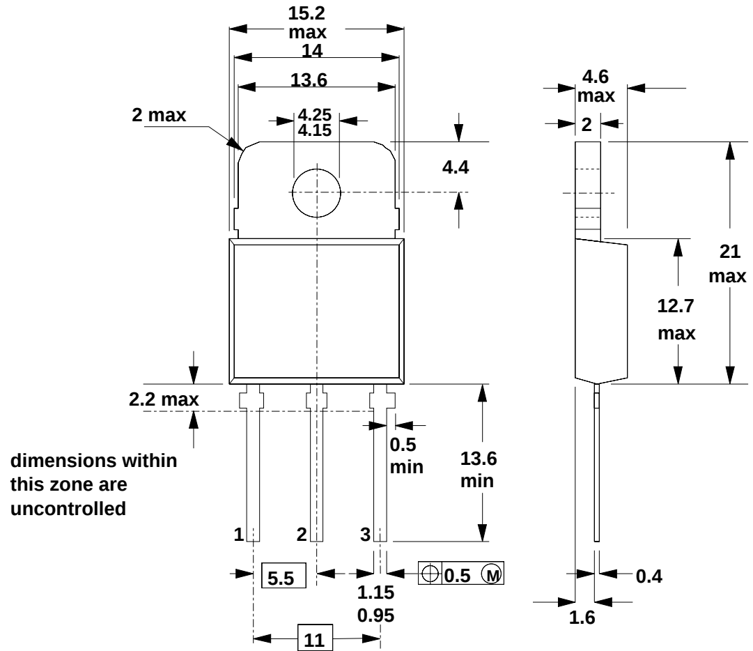
Fig.18. SOT93; pin 2 connected to mounting base.
