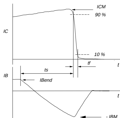
Fig.5. Switching times definitions.
