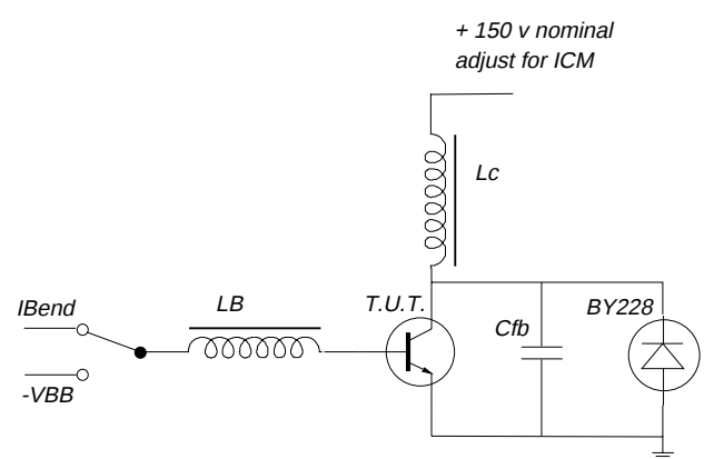
Fig.6. Switching times test circuit (BU2520A).
