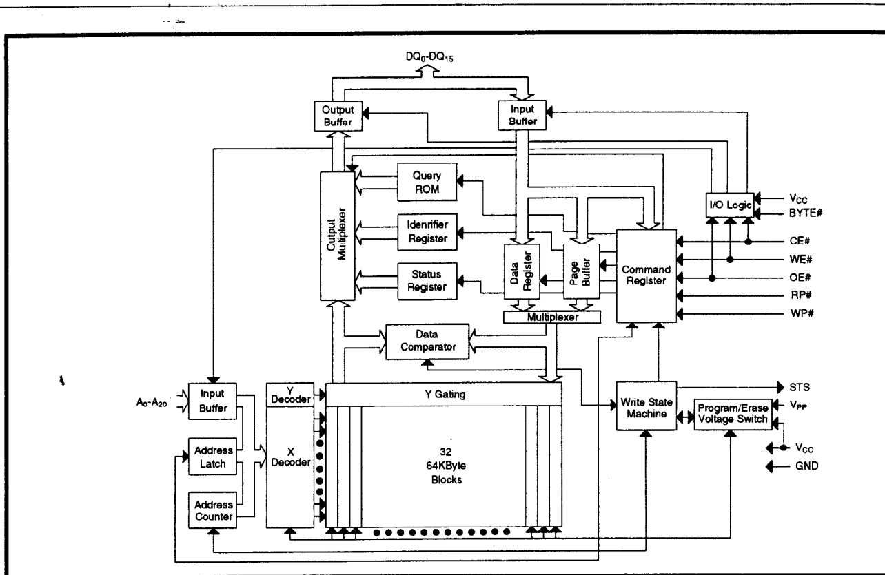
Figure 1. Block Diagram
