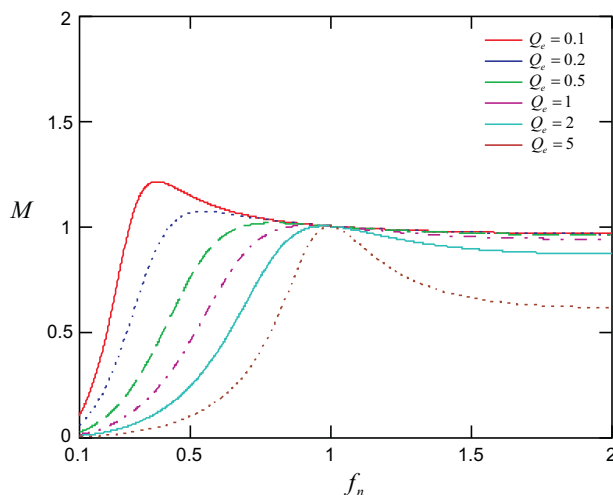
Figure 17. Normalized Switching Frequency vs. Converter Voltage Gain, L_n=20
