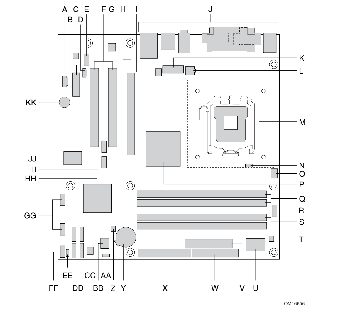
Figure 2. D915GAG Board Components
