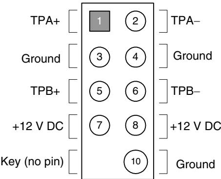
Figure 23. Connection Diagram for IEEE 1394a Connectors
