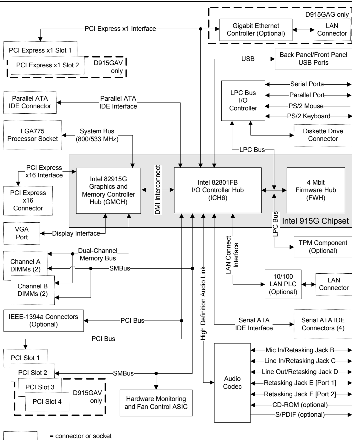
Figure 3. Block Diagram
