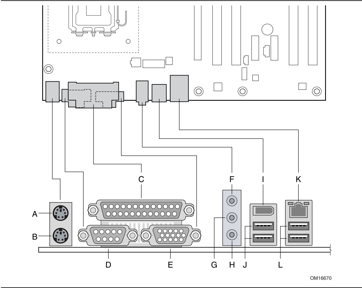
Figure 18. Back Panel Connectors
