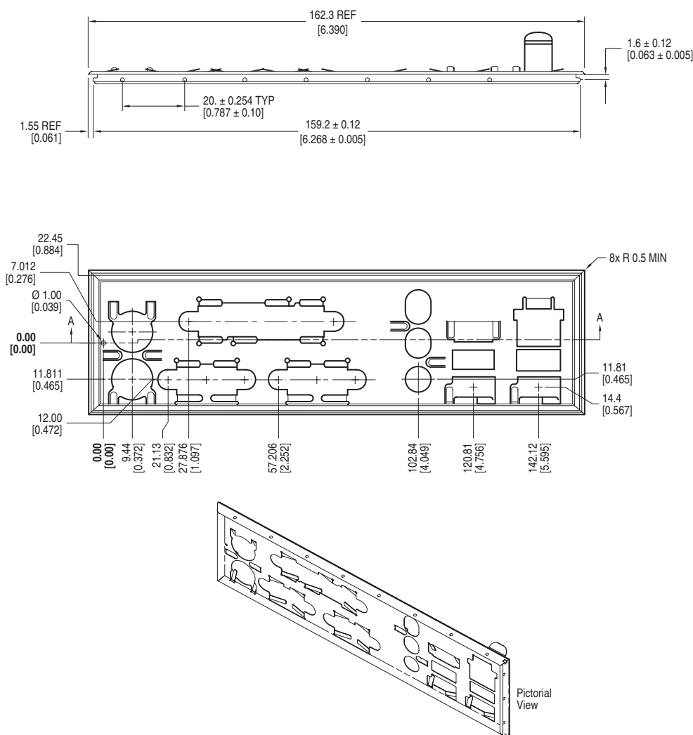
Figure 27. I/O Shield Dimensions
