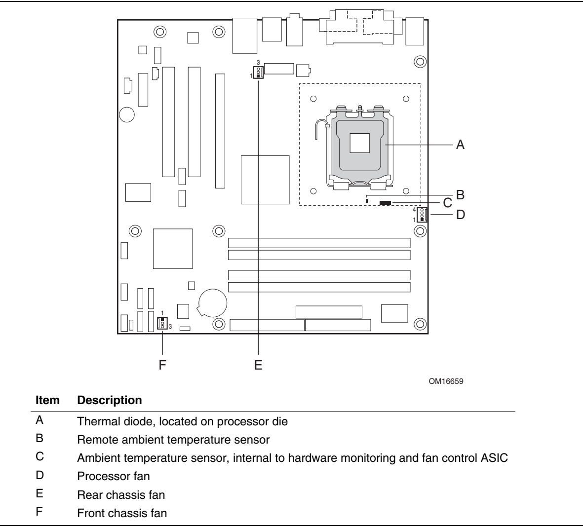
Figure 15. Thermal Monitoring for D915GAG Board
