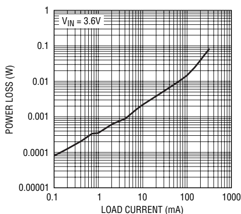
Figure 2. Power Loss vs Load Current
