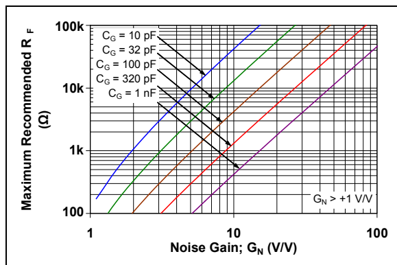
FIGURE 4-9: Maximum Recommended R_F vs. Gain.
