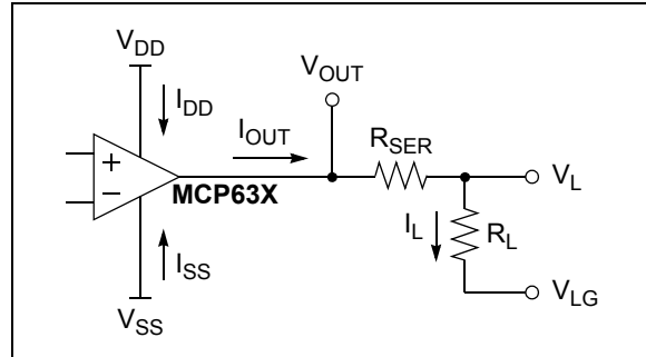
FIGURE 4-5: Diagram for Power Calculations.
