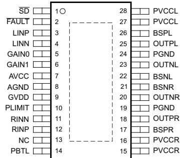
PWP Package 28-Pin HTSSOP With PowerPAD™ IC Package Top View
