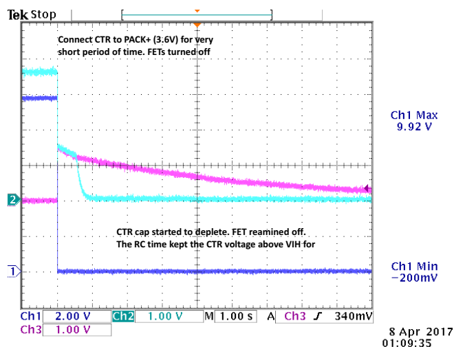
Figure 9-12. Setup CTR for System Shutdown (Using 5 M \Omega and 1 \mu F RC)
