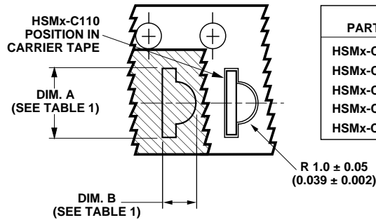
Figure 15. Tape dimensions.
