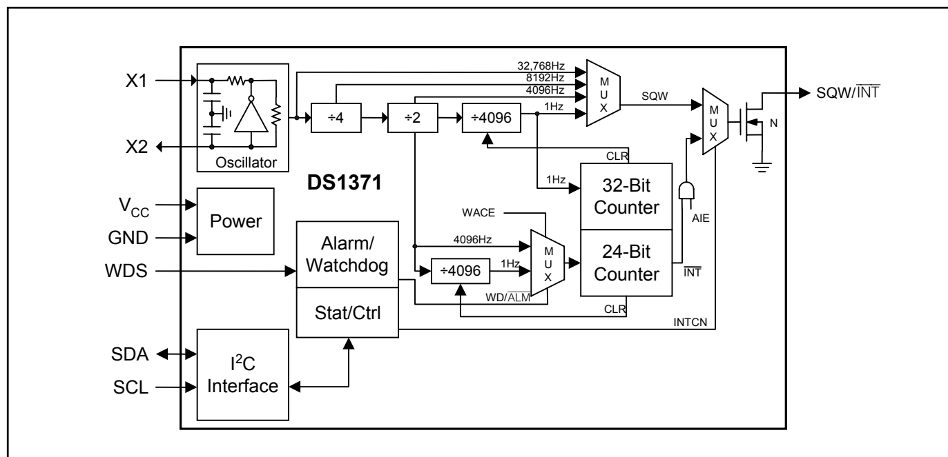
Figure 2. Functional Diagram
