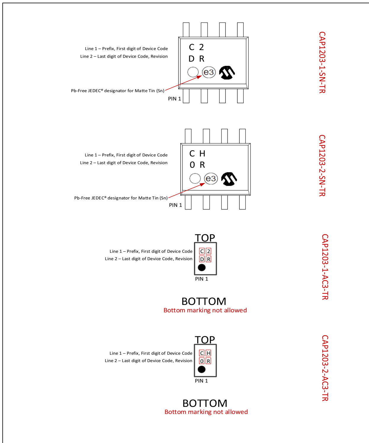
FIGURE 6-5: CAP1203 PACKAGE MARKING
