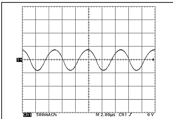
Figure 14: Input Terminal Ripple Current, i_c , at full rated output current and nominal input voltage with 3.3 \mu H source impedance and 100 \mu F electrolytic capacitor (500 mA/div). See Figure 13.
