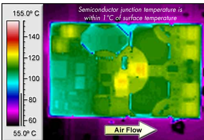
Figure 6: Thermal plot of converter at 20 amp load current with 55°C air flowing at the rate of 200 LFM. Air is flowing across the converter from input to output (nominal input voltage).
