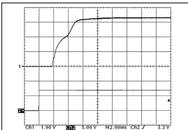
Figure 10: Turn-on transient at zero load (2 ms/div). Ch 1: V_{out} (1V/div). Ch 2: ON/OFF input (5V/div)
