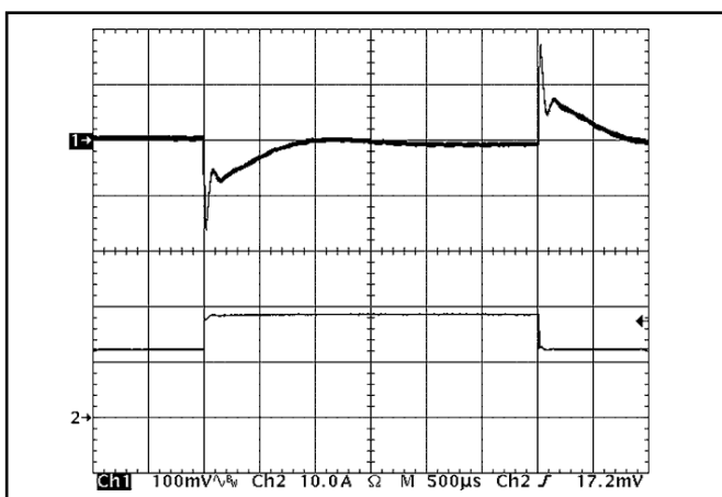
Figure 12: Output voltage response to step-change in load current (50%-75%-50% of I_{out(max)} ; dI/dt = 5A/\mu s ). Load cap: 470μF, 30 mΩ ESR tantalum capacitor and 1μF ceramic cap. Ch 1: V_{out} (100mV/div), Ch 2: I_{out} (10A/div).
