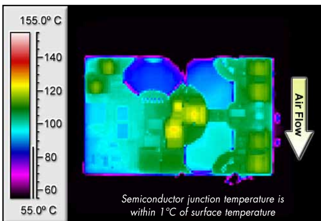
Figure 8: Thermal plot of converter at 19 amp load current with 55°C air flowing at the rate of 200 LFM. Air is flowing across the converter from pin 1 to pin 3 (nominal input voltage).
