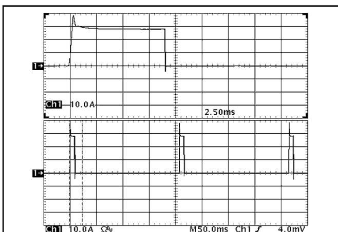
Figure 18: Load current (10A/div) as a function of time when the converter attempts to turn on into a 10 m \Omega short circuit. Top trace (2.5ms/div) is an expansion of the on-time portion of the bottom trace.
