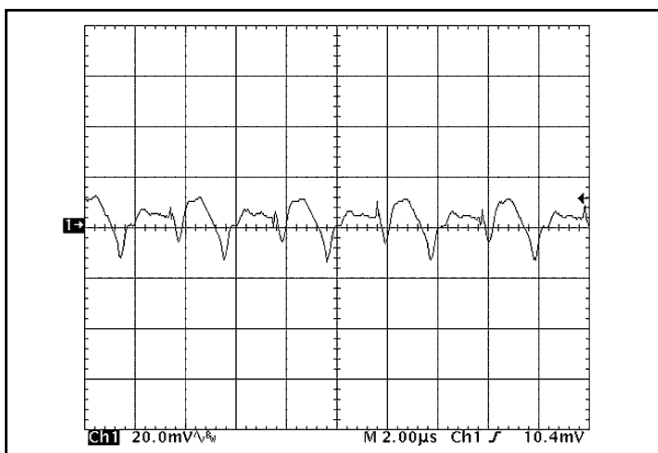
Figure 16: Output voltage ripple at nominal input voltage and rated load current (20 mV/div). Load capacitance: 1 \mu F ceramic capacitor and 10 \mu F tantalum capacitor. Bandwidth: 20 MHz. See Figure 13.
