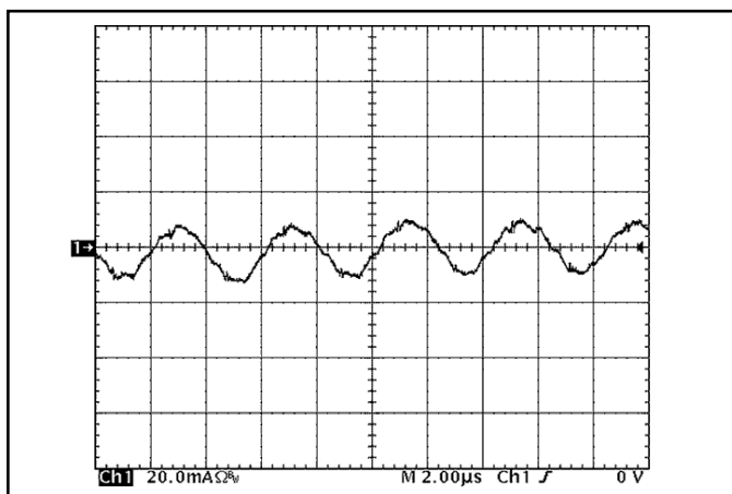
Figure 15: Input reflected ripple current, i_s , through a 3.3 \mu H source inductor at nominal input voltage and rated load current (20 mA/div). See Figure 13.
