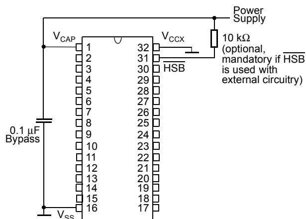
Figure 2: DISABLING AUTOMATIC STORES Schematic Diagram
