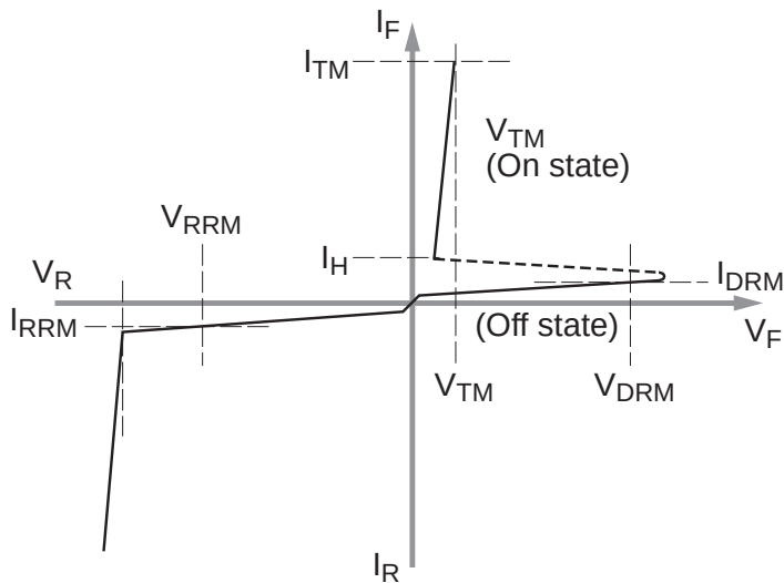
Voltage-Current Characteristic
