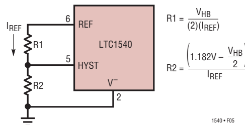
Figure 5. Programmable Hysteresis
