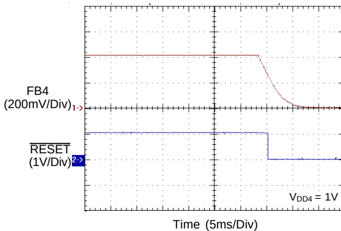
\overline{\text{RESET}} Power Off
