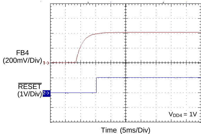
\overline{\text{RESET}} Power On
