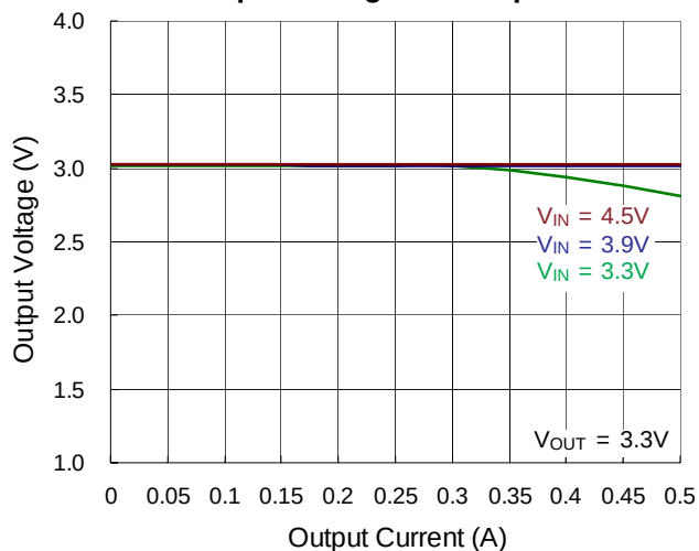
CH3 Output Voltage vs. Output Current
