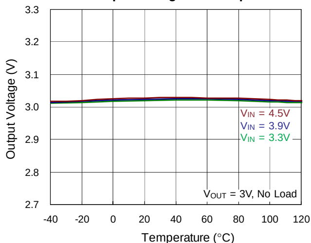
CH3 Output Voltage vs. Temperature
