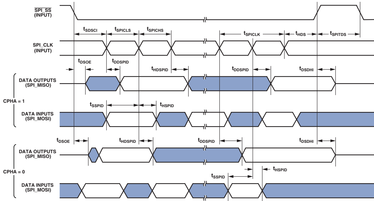
Figure 41. Serial Peripheral Interface (SPI) Port—Slave Timing
