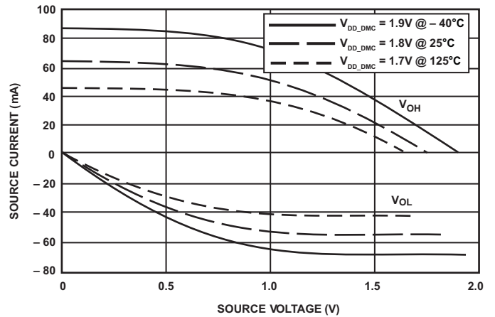
Figure 61. Driver Type B Current ( 1.8\text{ V } V_{DD\_DMC} )
