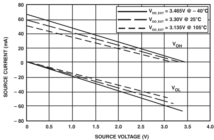
Figure 60. Driver Type A Current ( 3.3\text{ V } V_{DD\_EXT} )
