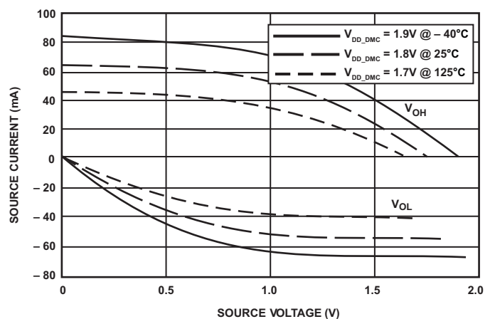
Figure 62. Driver Type C Current ( 1.8\text{ V } V_{DD\_DMC} )
