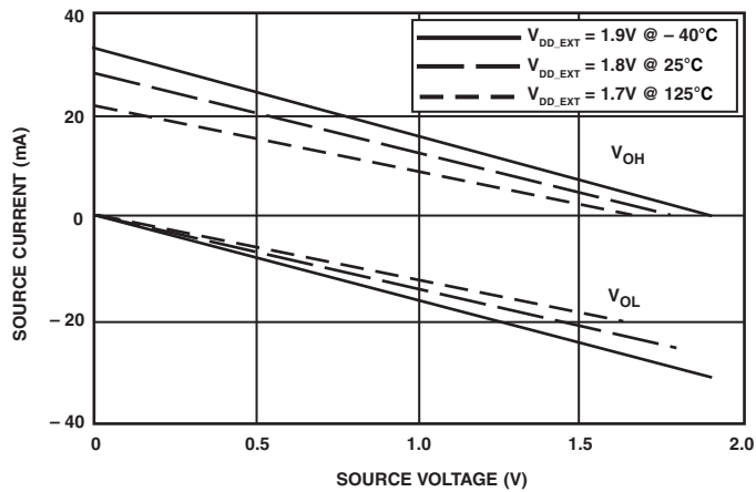
Figure 59. Driver Type A Current ( 1.8\text{ V } V_{DD\_EXT} )
