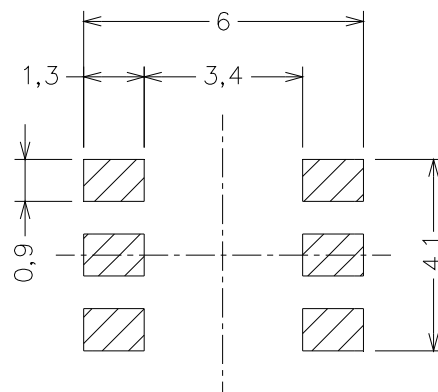
Soldering patterns
