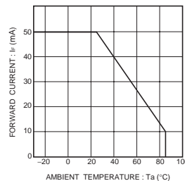
Fig.2 Forward current falloff
