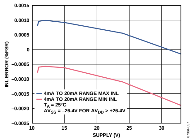
Figure 43. Integral Nonlinearity Error vs. AV_{DD}/|AV_{SS}| , Over Supply, Internal R_{SET}
