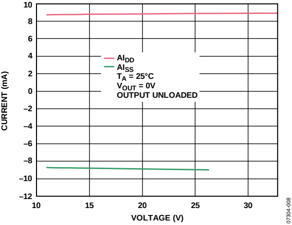
Figure 67. A_{ID}/A_{IS} vs. AV_{DD}/AV_{SS}
