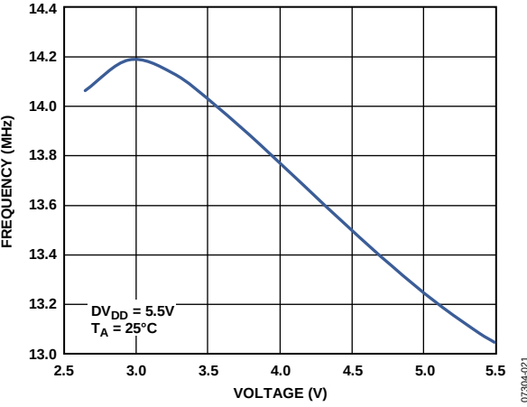
Figure 70. Internal Oscillator Frequency vs. DV_{DD} Supply Voltage
