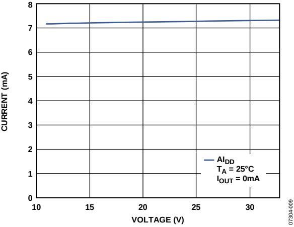
Figure 68. A_{ID} vs. AV_{DD}
