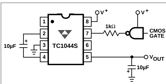
Figure 6. External Clocking
