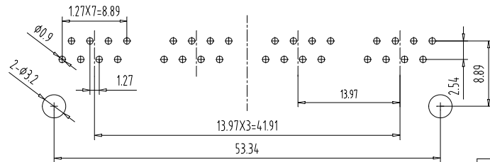
PC Board Layout Component Side Shown
