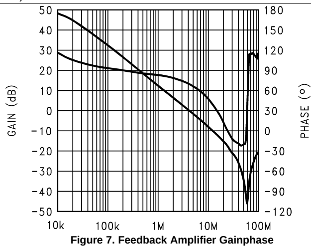
Figure 7. Feedback Amplifier Gainphase
