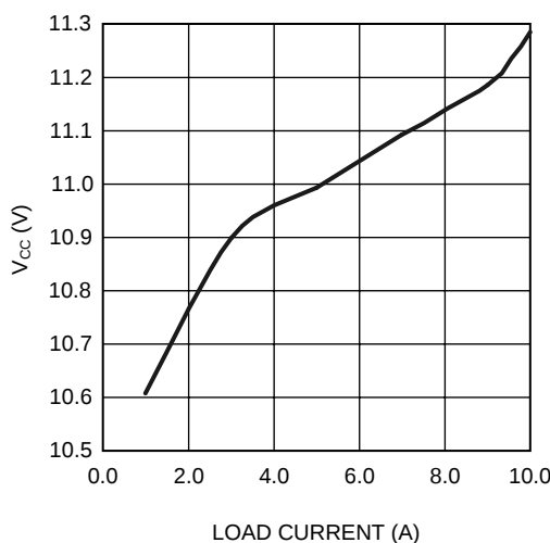
Figure 9. V_{CC} Voltage vs Load Current
