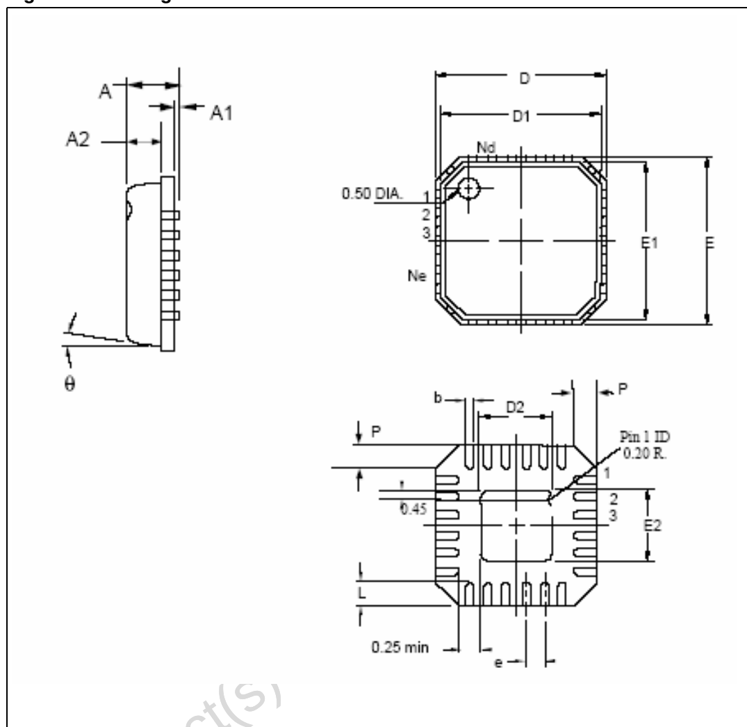
Figure 23. Package dimensions
