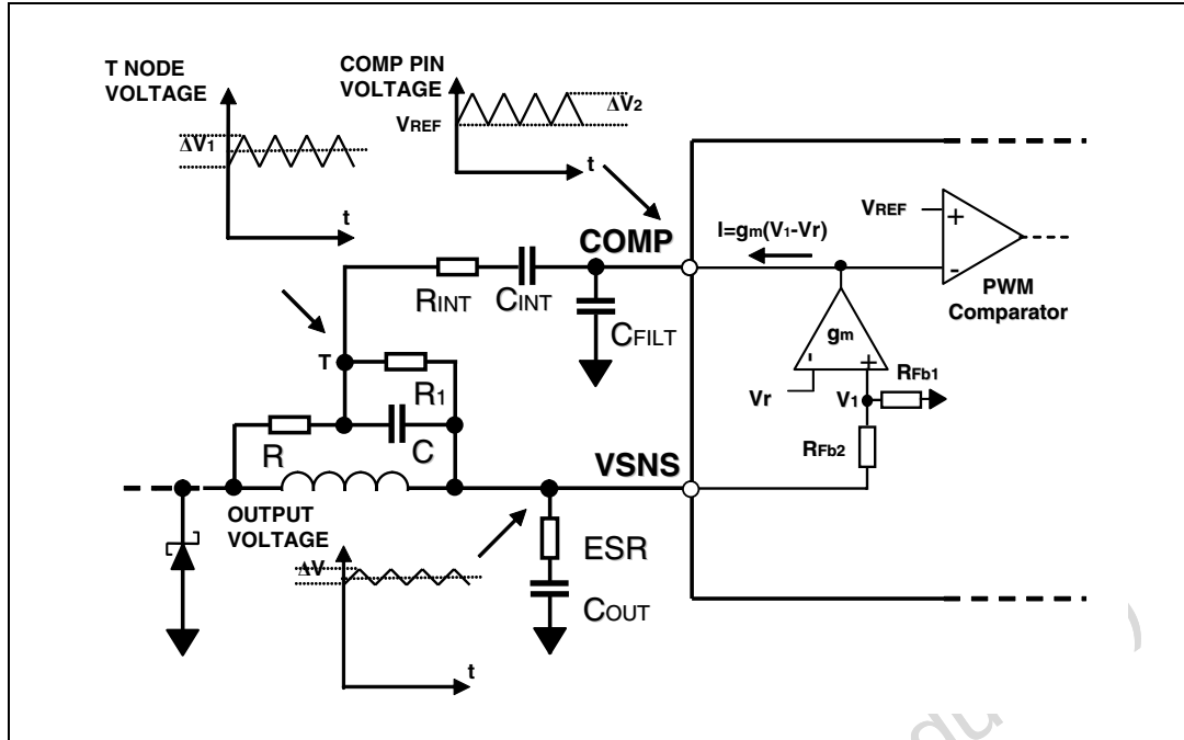
Figure 8. "Virtual-ESR" network
