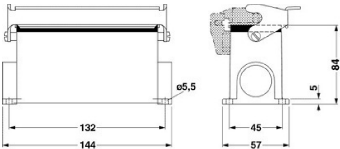
Dimensioned drawing
