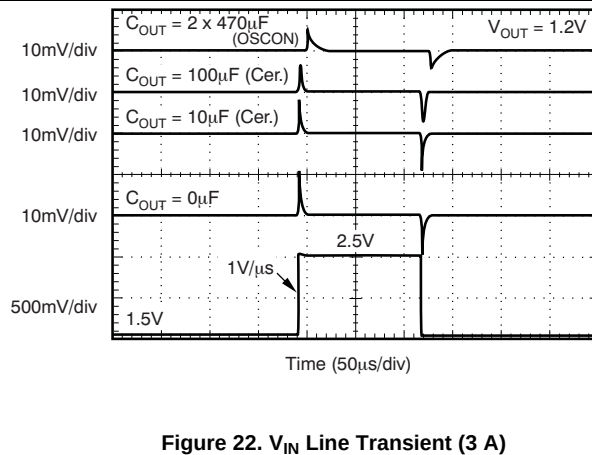
Figure 22. V_{IN} Line Transient (3 A)
